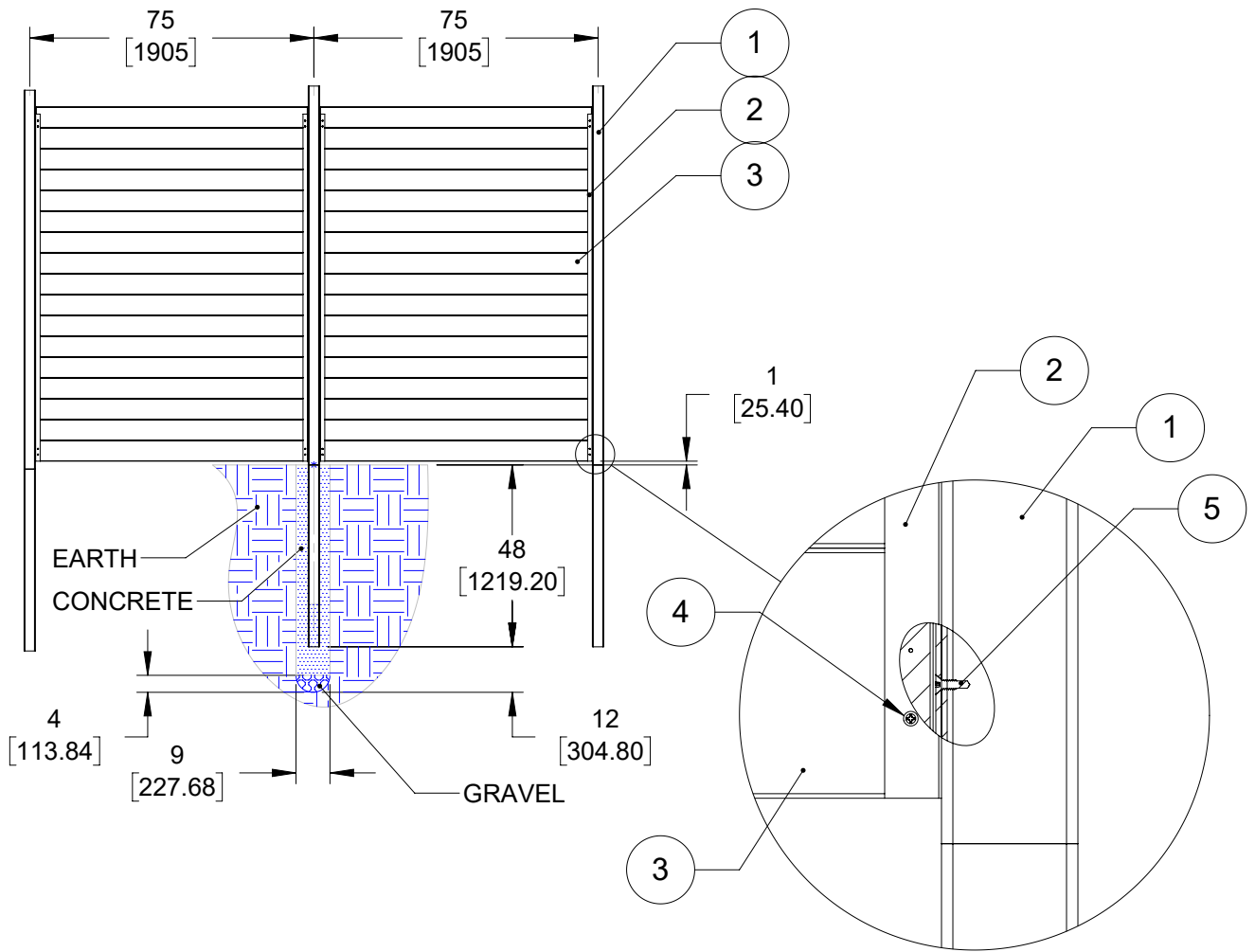
DETAIL C SCALE 1 : 4
